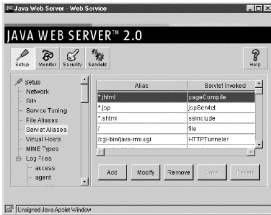
Figure 22-2. Sun's JavaWebServer
