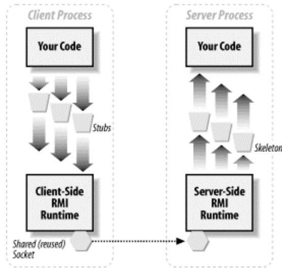
Figure 16-2. Sharing sockets
