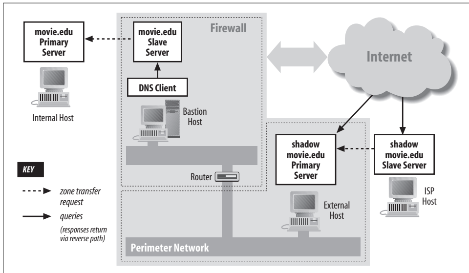
Figure 11-6. A split DNS solution
