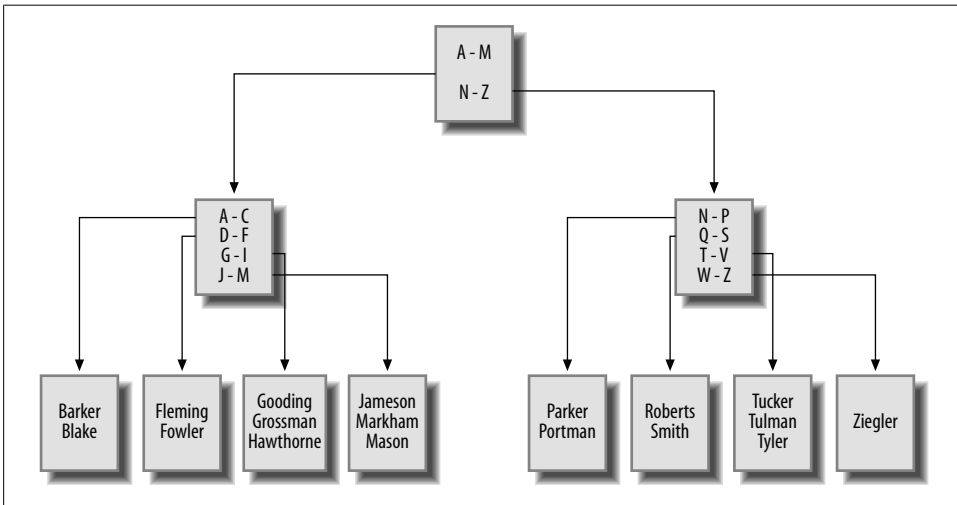
Figure 13-1. B-tree example
